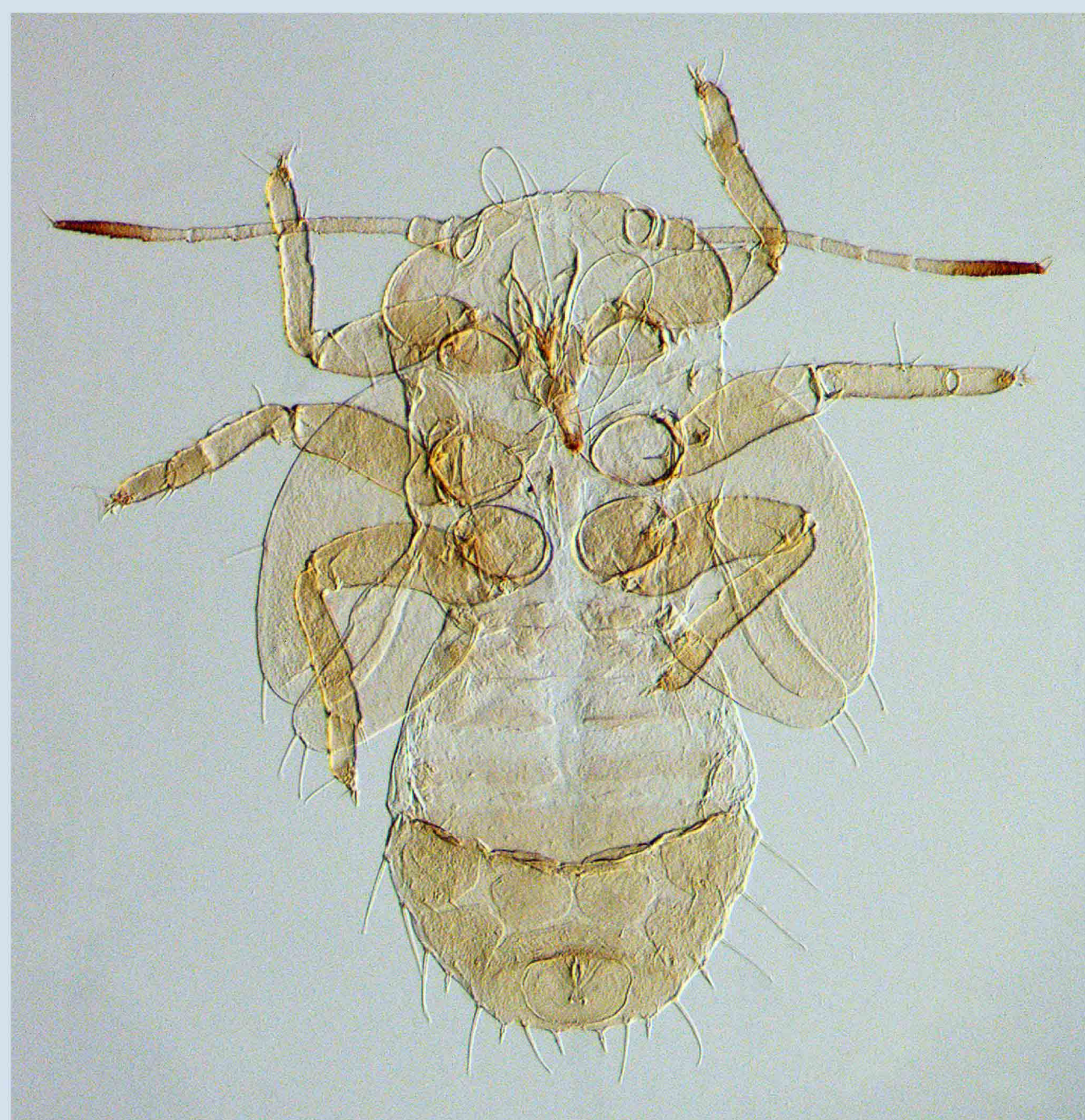
Larve
